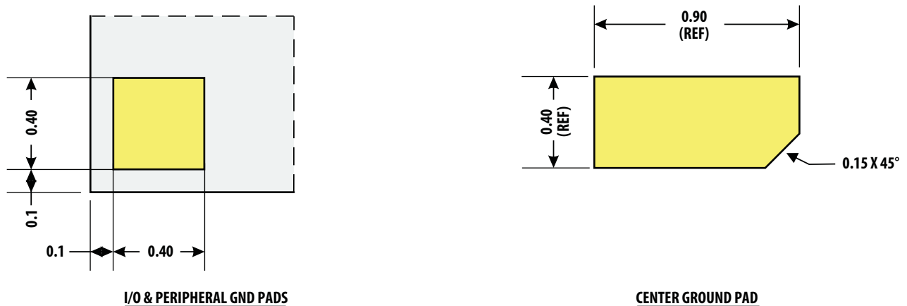
Figure 18. Pad Detail
