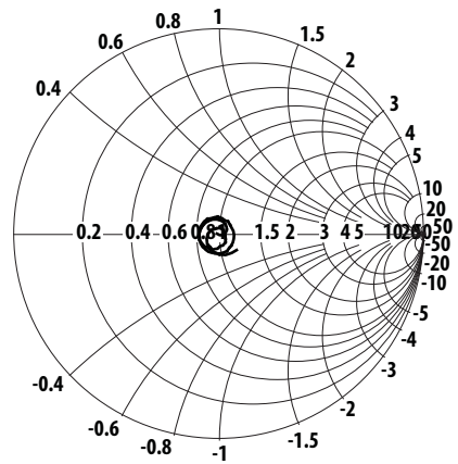
Figure 16. Ant Port Impedance in Rx Band
