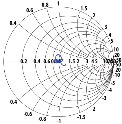
Figure 14. Rx Port Impedance in Rx Band
