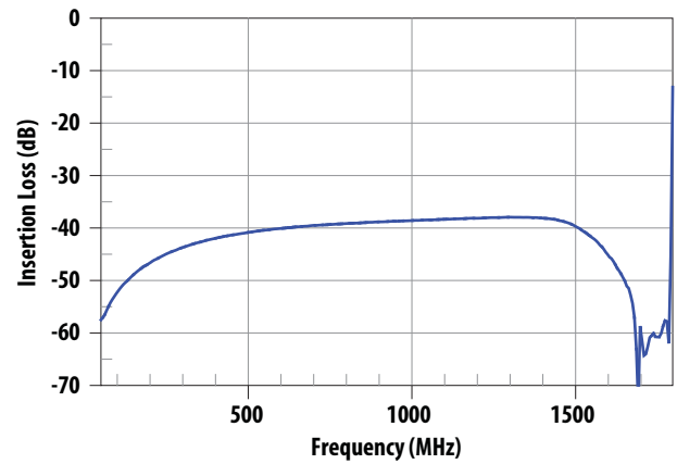
Figure 10. Ant-Rx Low Frequency Rejection, 50 – 1800 MHz
