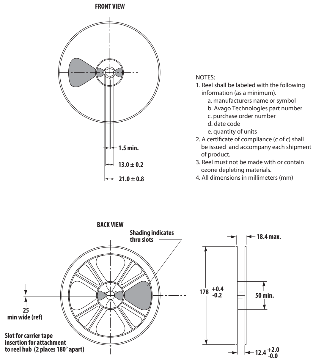
Figure 29. SMT Reel Drawing
